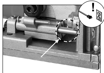
Fig. 27. Location of sliding base guide rail (1 of 2).
